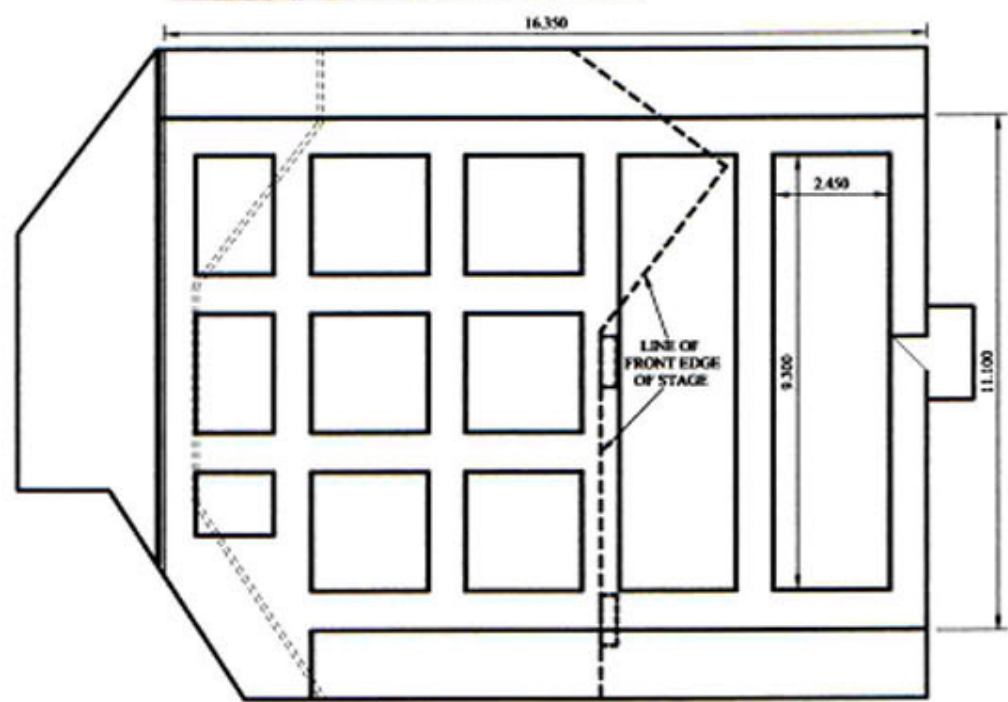
HIGH LEVEL LIGHTING & CATWALK LAYOUT 1:100
