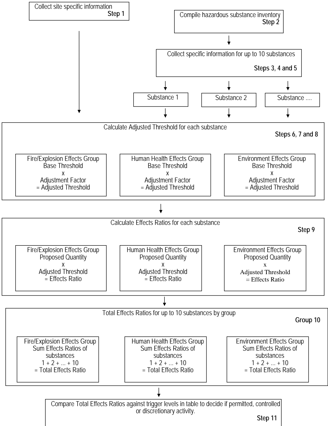
FIGURE 1 - HAZARDOUS FACILITY SCREENING PROCEDURE - OVERVIEW
