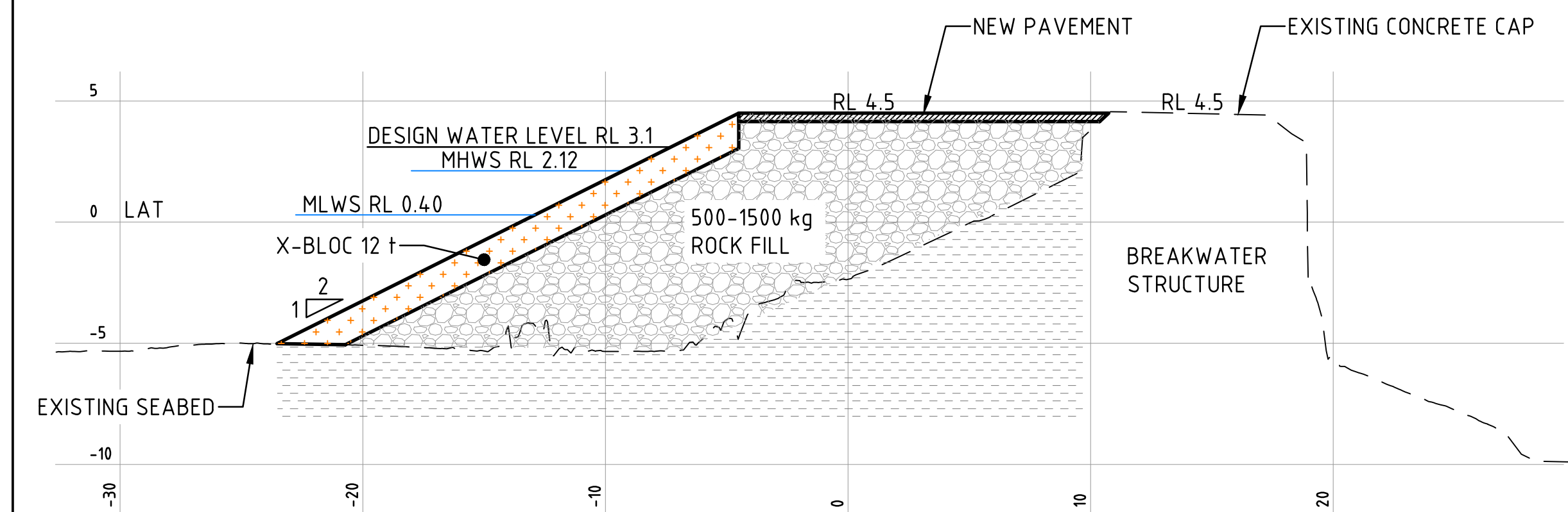
SECTION A-A SCALE 1:200 (A1)
