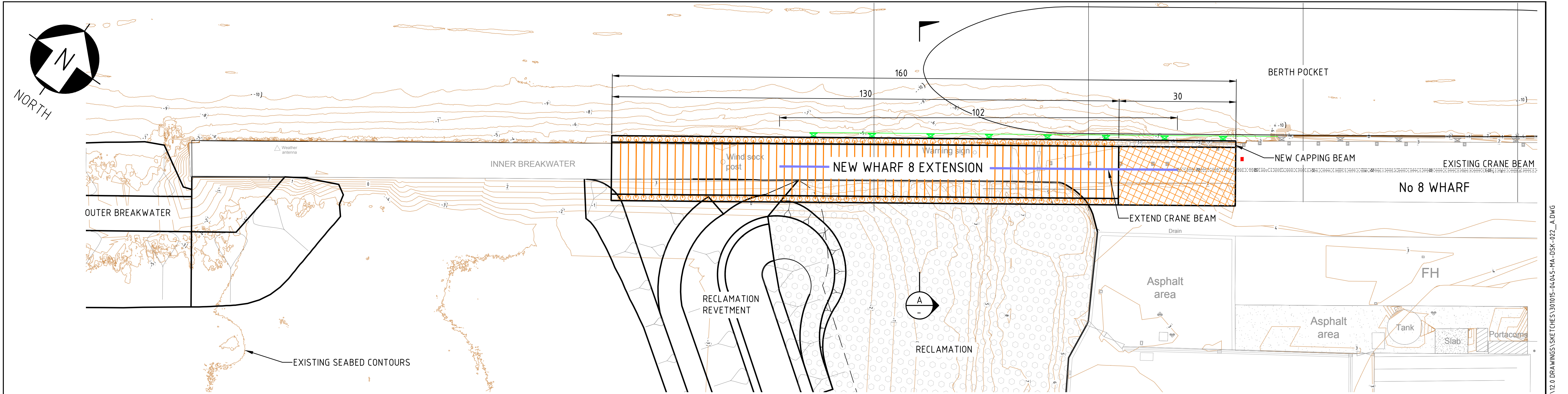
GENERAL ARRANGEMENT SCALE 1:500 (A1)
