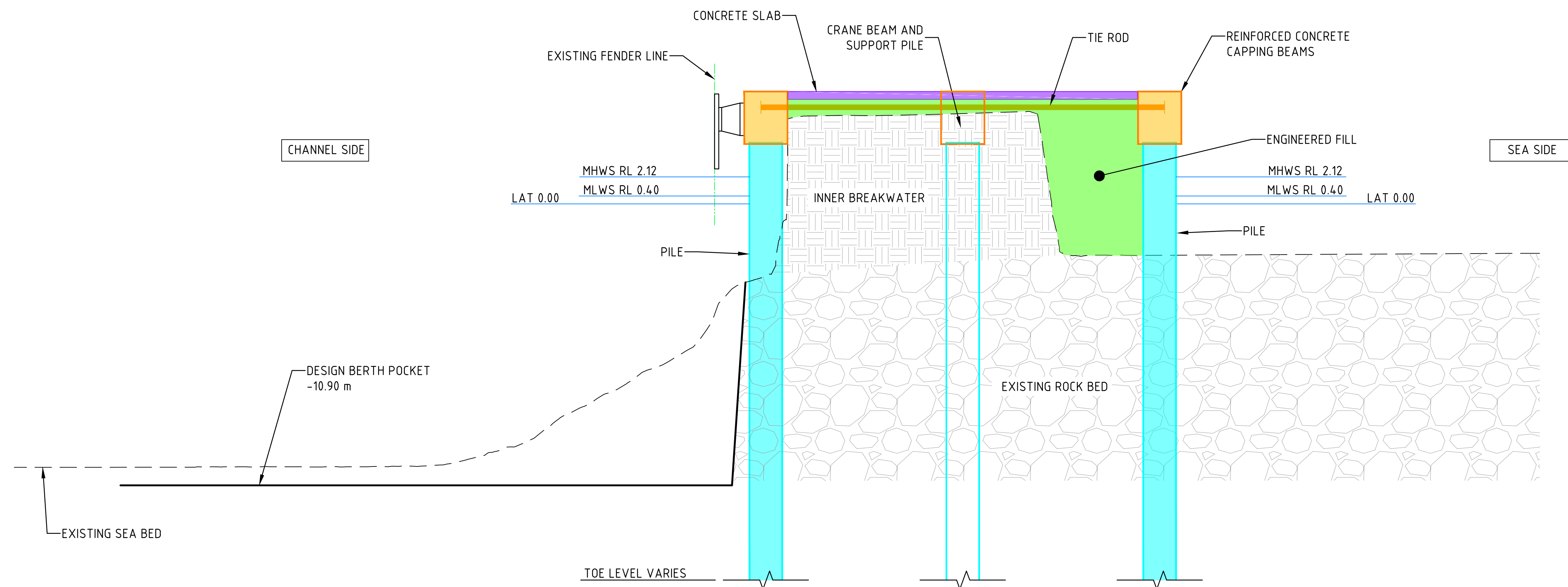
SECTION A 022 (REVTMENT NOT SHOWN IN THIS SECTION FOR CLARITY)
