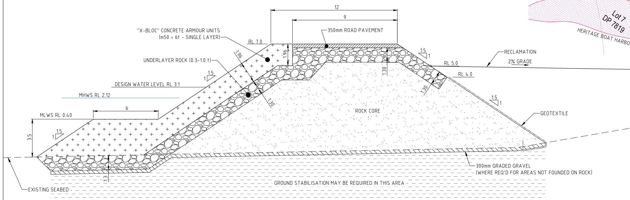
RECLAMATION REVETMENT - TYPICAL SECTION SCALE 1:100 (A1)
