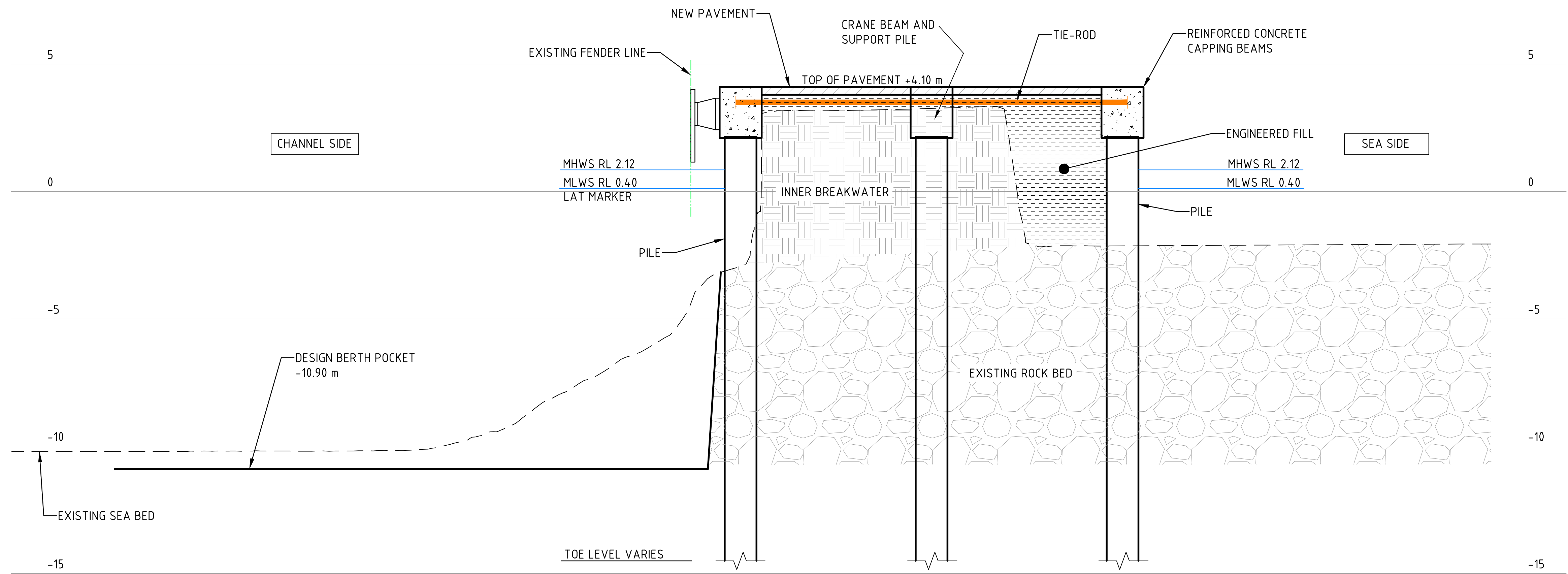
SECTION A-A (REVETMENT NOT SHOWN IN THIS SECTION FOR CLARITY) SCALE 1:100 (A1)
