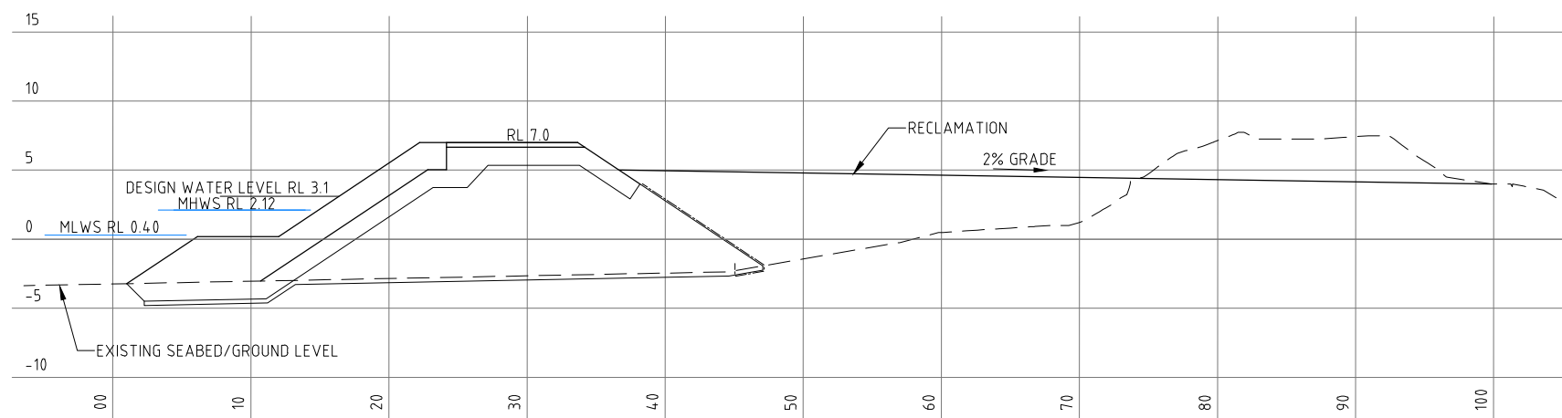
SECTION A SCALE 1:250 (A1) -
