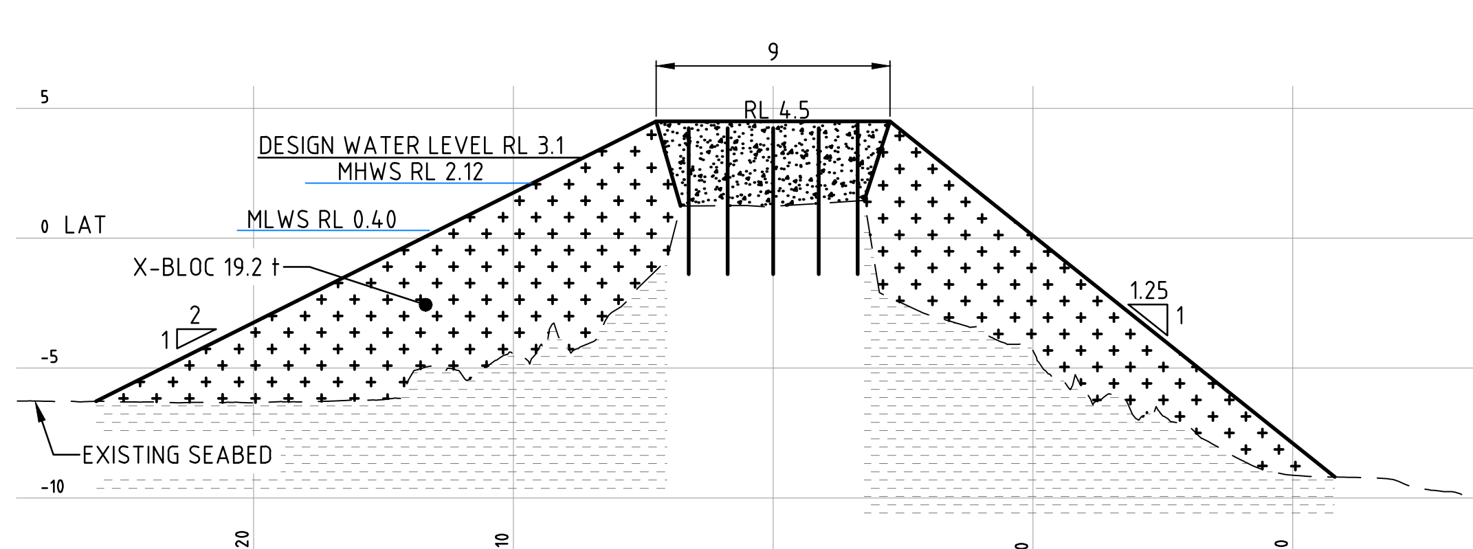
SECTION C-C SCALE 1:200 (A1)
