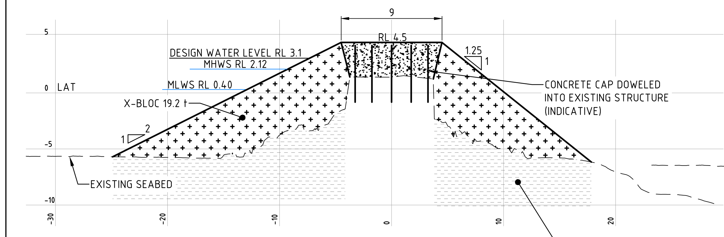
SECTION B-B SCALE 1:200 (A1)
