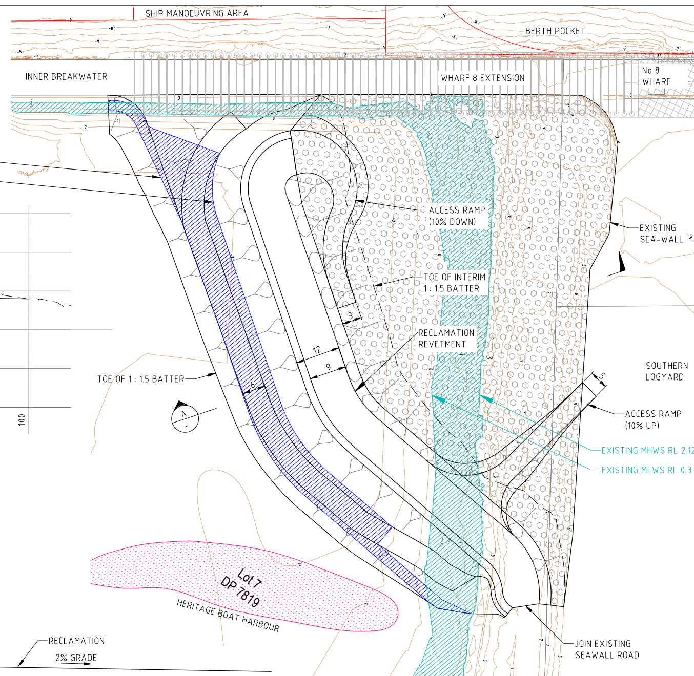
GENERAL ARRANGEMENT SCALE 1:500 (A1)
