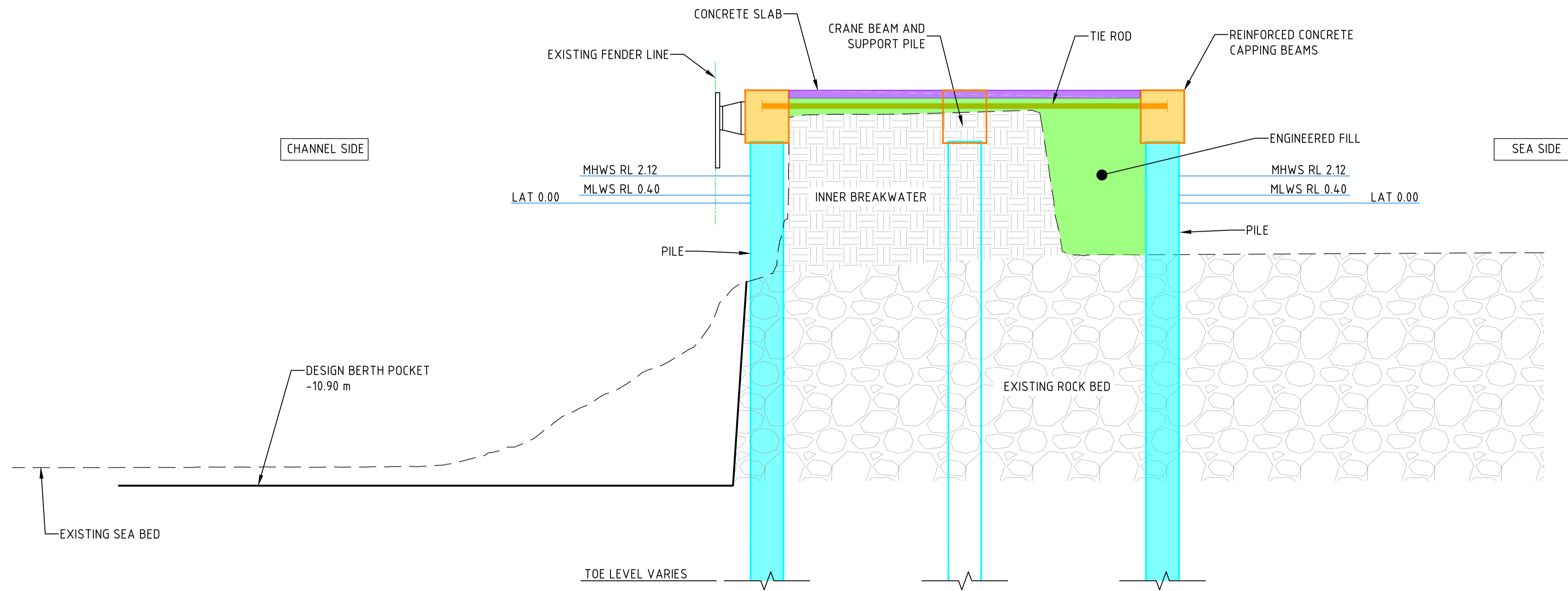
SECTION A SCALE 1:100 (A1) 022 (REVETMENT NOT SHOWN IN THIS SECTION FOR CLARITY)
